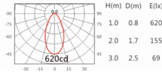
CITIZEN COB 45° 3000K
