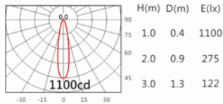
CITIZEN COB 20° 3000K
