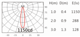
CITIZEN COB 20° 4000K
