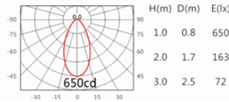
CITIZEN COB 45° 4000K
