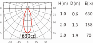
CITIZEN COB 35° 2700K
