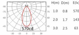
CITIZEN COB 45° 2700K
