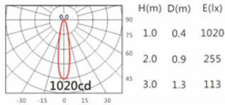
CITIZEN COB 20° 2700K
