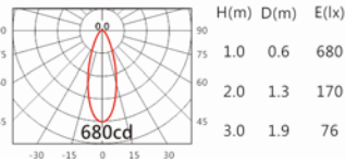
CITIZEN COB 35° 3000K
